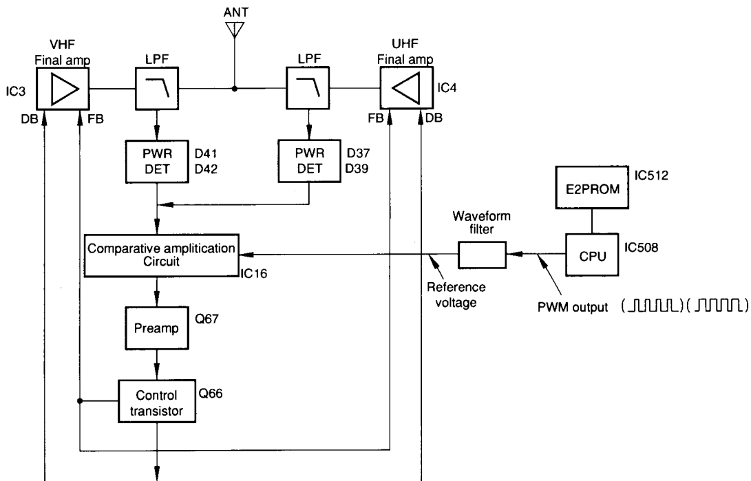
Fig.2 APC circuit
