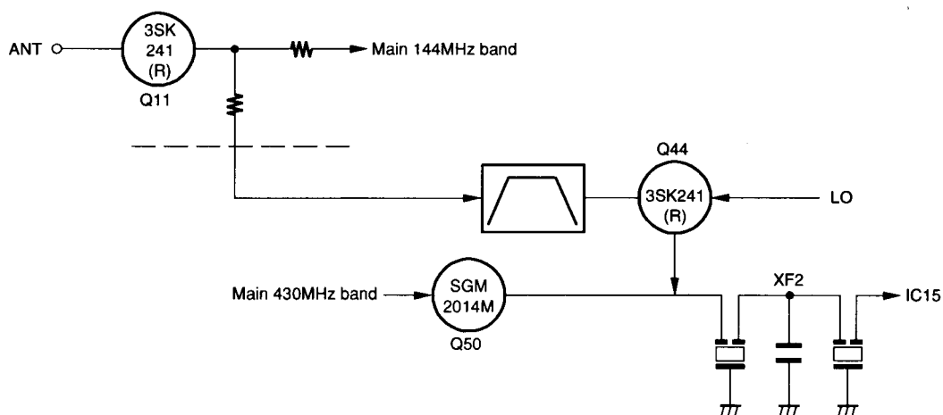
Fig.3 144MHz sub band receive circuit block diagram
